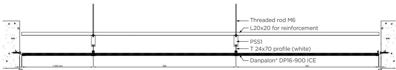
Cut A-A: on reinforcement area
