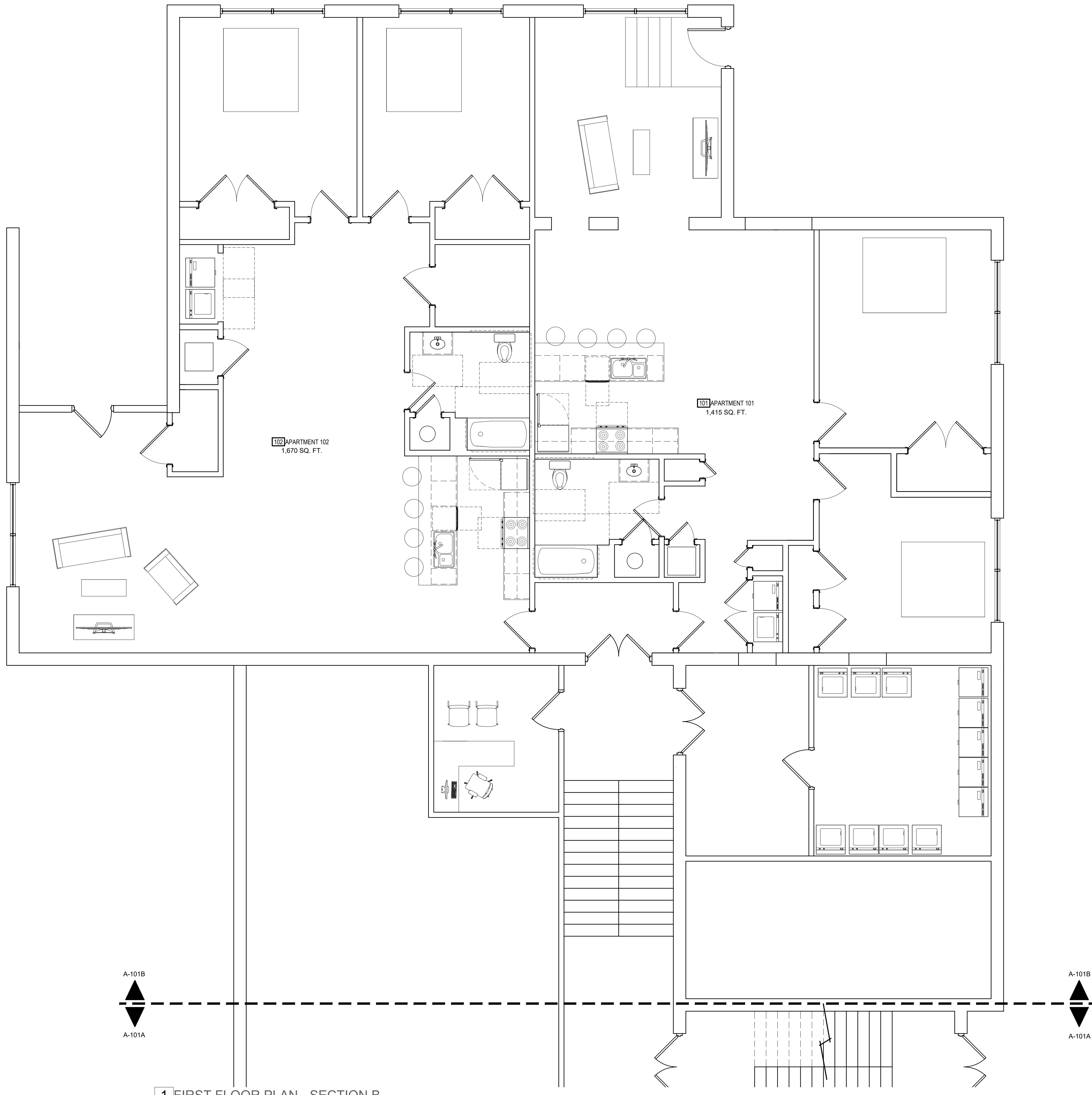
1 FIRST FLOOR PLAN - SECTION B. A-101B 1/4" = 1'-0"
