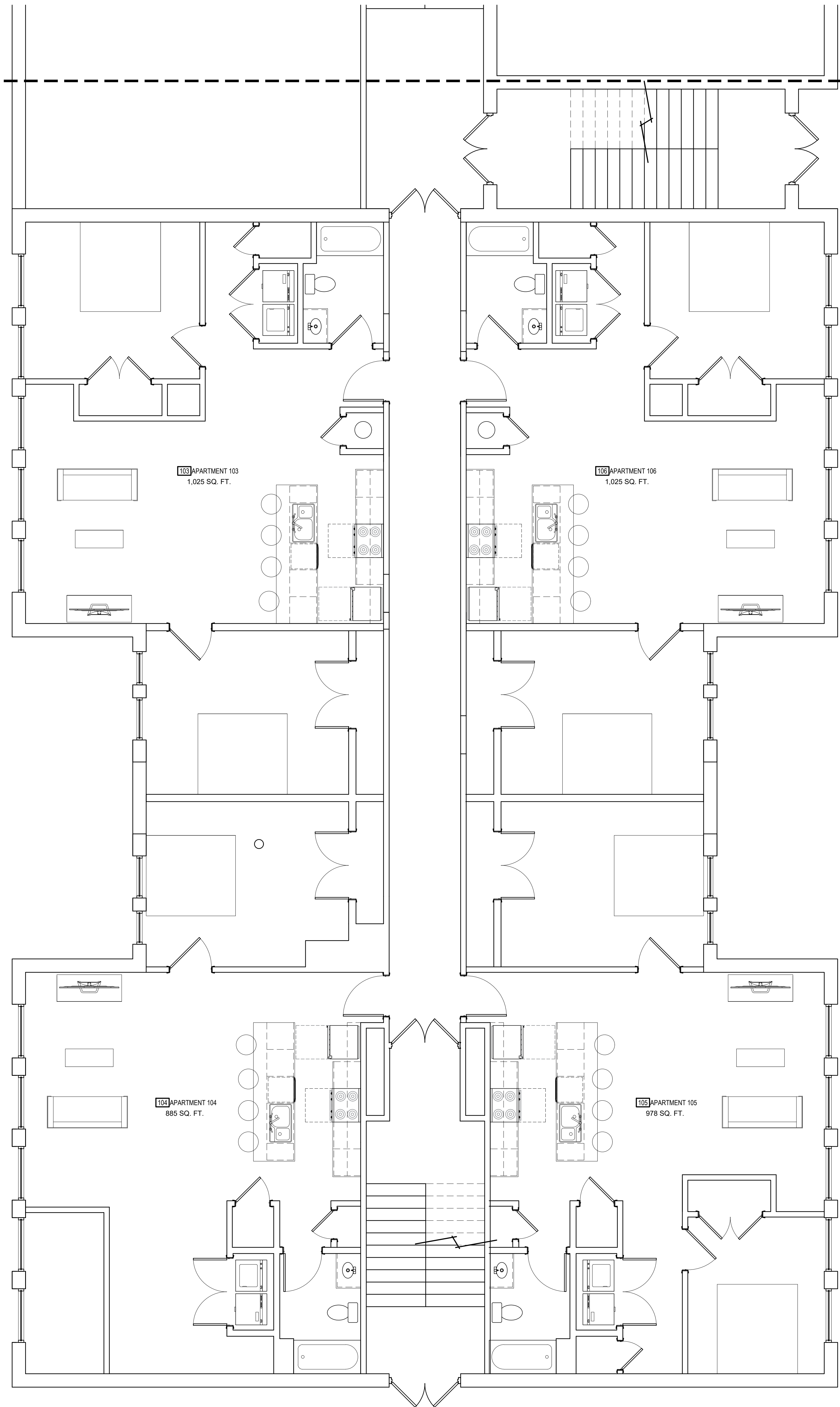
1 FIRST FLOOR PLAN - SECTION A
