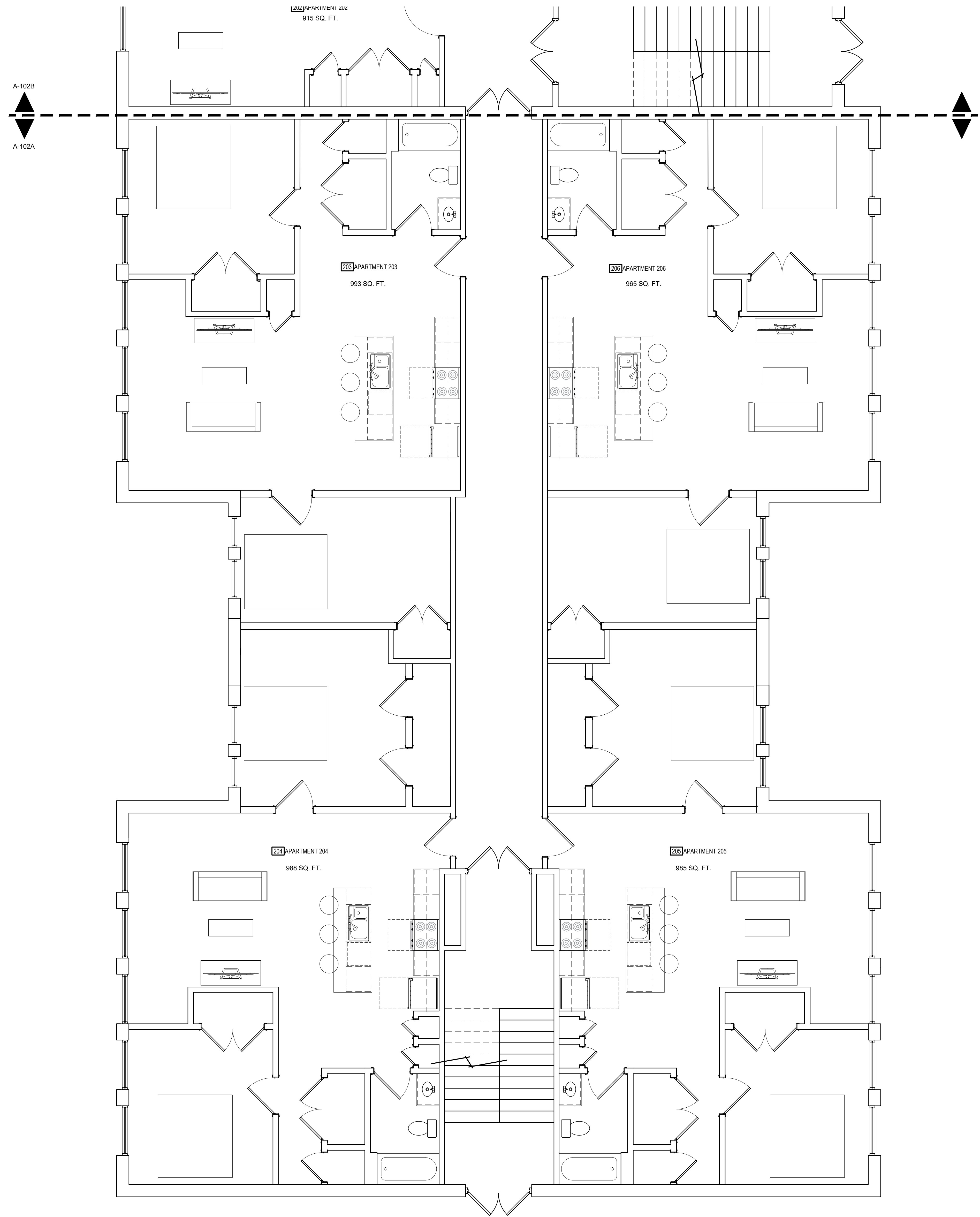
1 SECOND FLOOR PLAN - SECTION A A-102A 1/4" = 1'-0"
