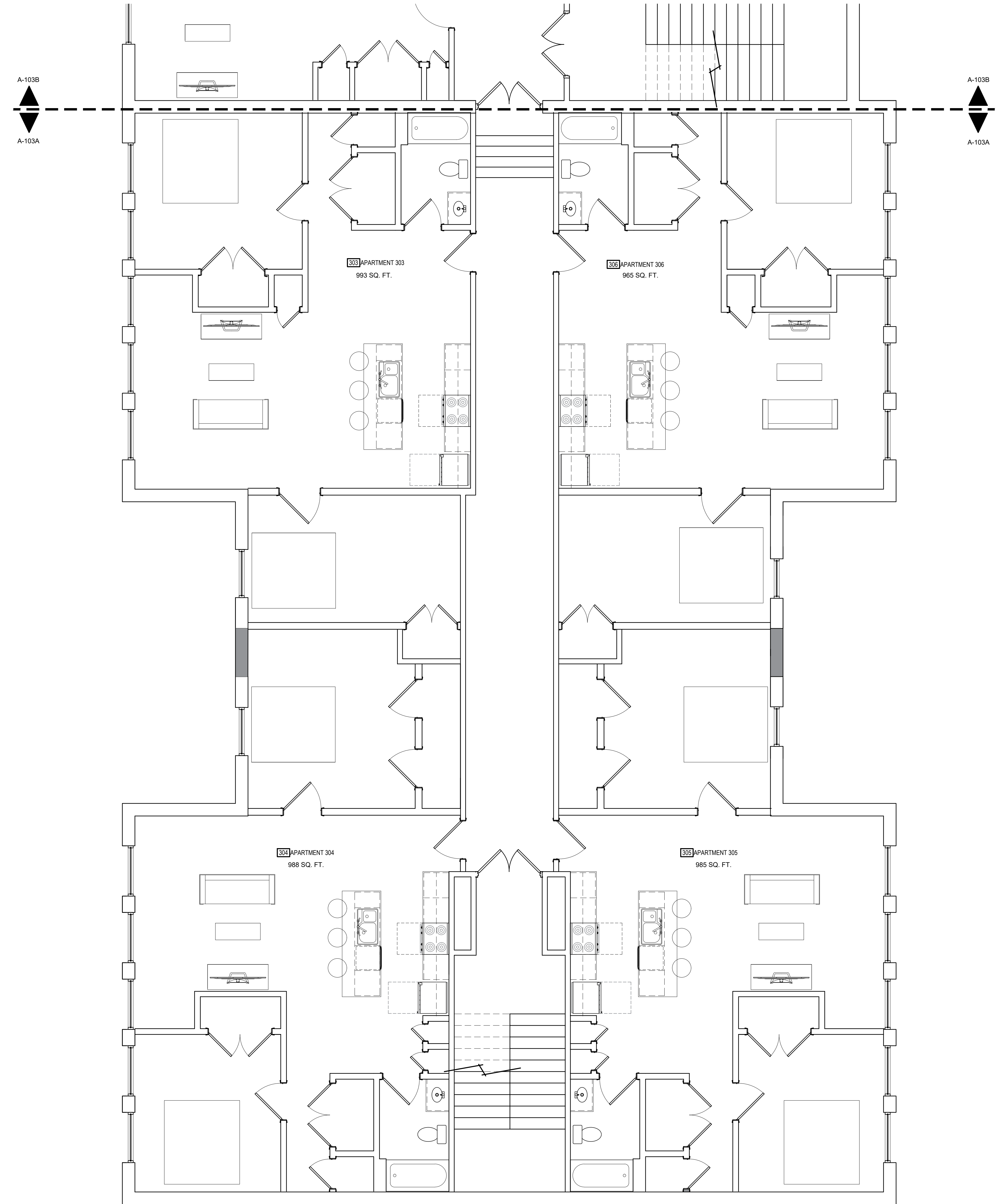
1 THIRD FLOOR PLAN - SECTION A A-103A 1/4" = 1'-0"
