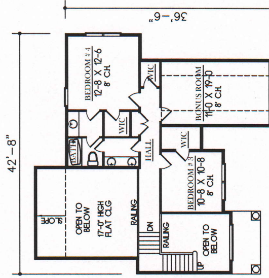
SECOND FLOOR = 586 SQ. FT.
