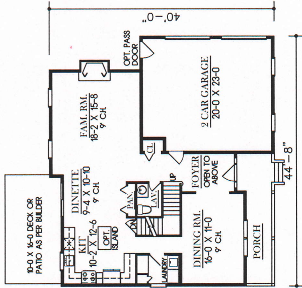
FIRST FLOOR = 1049 SQ. FT.
