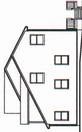
LEFT ELEVATION
