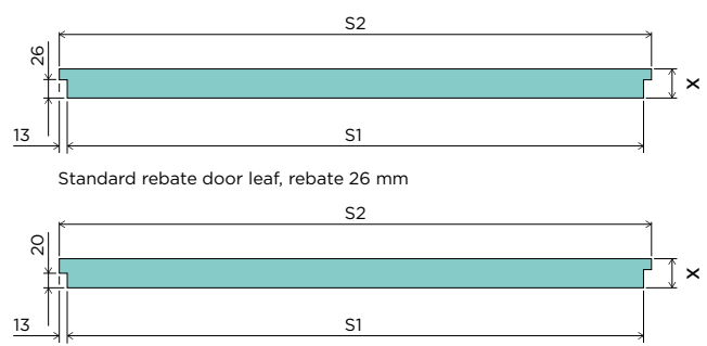
20 mm rebate door leaf OPTIONAL
