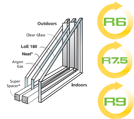
R6 Triple Pane, LoE 180 Neat®, Argon with Super Spacer R7.5 Triple Pane, LoE 180 Neat®, 50% Argon/50% Krypton with Super Spacer R9 Triple Pane, LoE 180 Neat®, Krypton with Super Spacer
