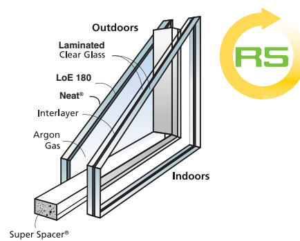
R5 Laminated, LoE 180 Neat®, Argon with Super Spacer
