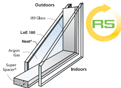
R5 LoE 180 Neat® with i89 Argon with Super Spacer
