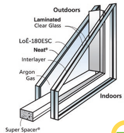
LAMINATED GLASS
