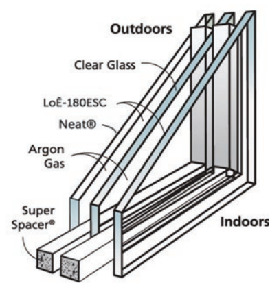
TRIPLE PANE
