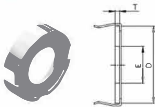
Gasket Retainer
