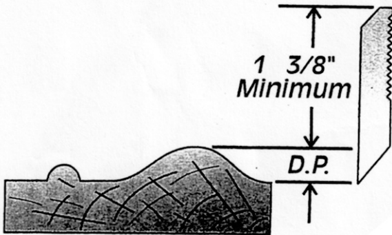
TOP (OR RIGHT) CUTTERHEAD
