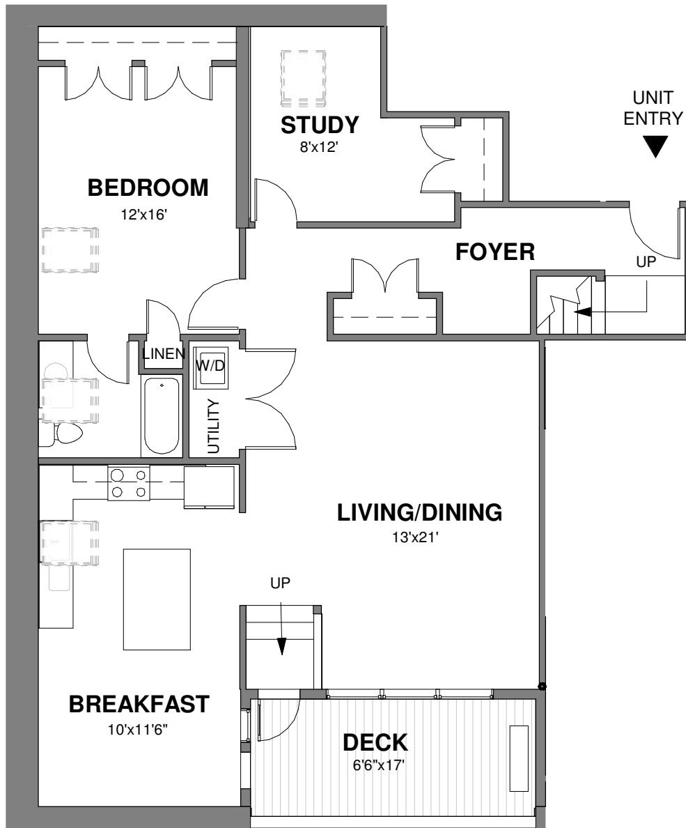
DUPLEX LOWER LEVEL 1,338 SF
