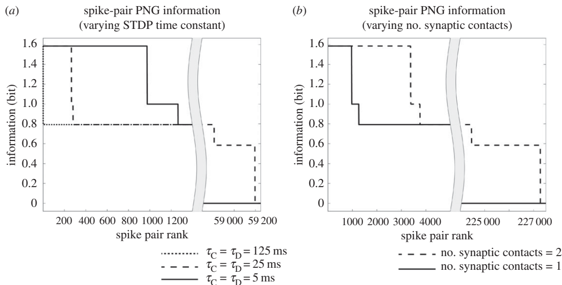
Figure 13. (a) Effect of varying the STDP time constants. Eguchi et al. [9] analysed how the stimulus information carried by spike-pair PNGs in the output layer was affected by varying the STDP time constants across the range \tau_C = \tau_D = 125 ms, 25 ms or 5 ms. It was found that the network developed the most spike-pair PNGs carrying maximal information about stimulus identity when the STDP time constants were shortest. Short STDP time constants maintain the temporal precision of the STDP, which is required to promote the development of stimulus-specific PNGs. (b) Effect of varying the number of synaptic connections between each pair of pre- and postsynaptic excitatory neurons. The original study also analysed how varying the number of synaptic connections between each pair of pre- and postsynaptic neurons affected the stimulus information carried by spike-pair PNGs in the output layer. Results are shown for simulations with either one or two connections between each pair of pre- and postsynaptic neurons. In the case of two synaptic connections, the contacts are assigned different axonal delays chosen randomly in the interval [0, 10] ms. This allows the STDP to selectively strengthen one connection with a particular axonal delay instead of the other connection with a different delay in order to promote the development of PNGs within the network. Indeed, it can be seen that far more PNGs carrying maximal stimulus information emerge in the simulations with two connections between each pair of pre- and postsynaptic neurons. Copyright © 2018 American Psychological Association. Reproduced [or Adapted] with permission. The official citation that should be used in referencing this material is [9]. No further reproduction or distribution is permitted without written permission from the American Psychological Association.
