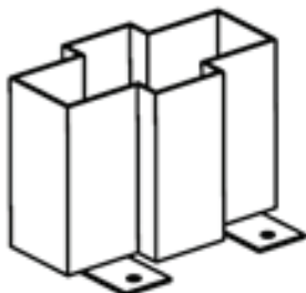
MBR REVERSE MULLION BASE ANCHOR
