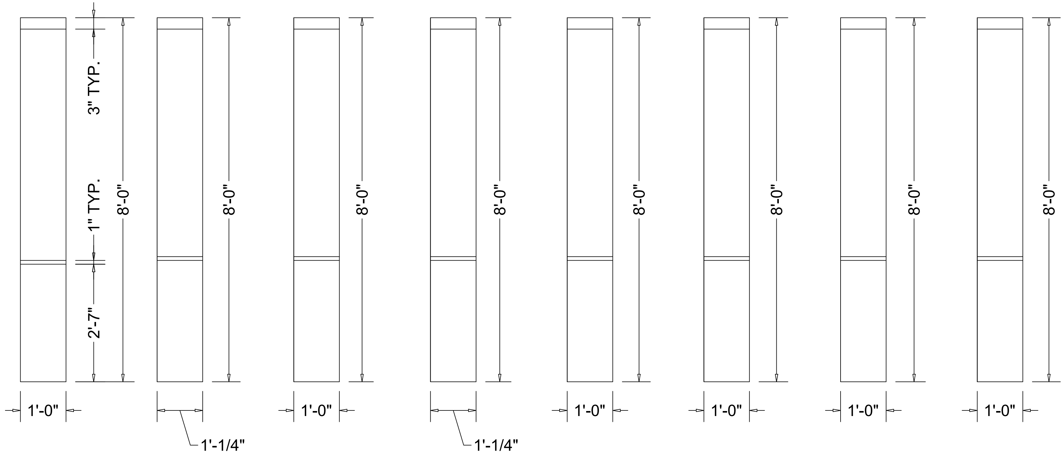
ELEVATION PILLAR (A1) ELEVATION PILLAR (A2) ELEVATION PILLAR (A3) ELEVATION PILLAR (A4) ELEVATION PILLAR (B1) ELEVATION PILLAR (B2) ELEVATION PILLAR (B3) ELEVATION PILLAR (B4)
