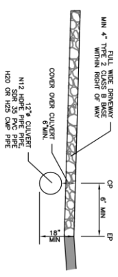
CULVERT LOCATION
