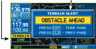
TERRAIN Annunciation and Pop-Up Alert
