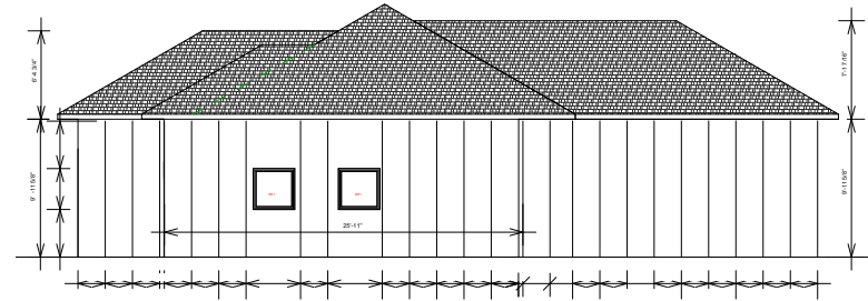
EAST SIDE ELEVATION
