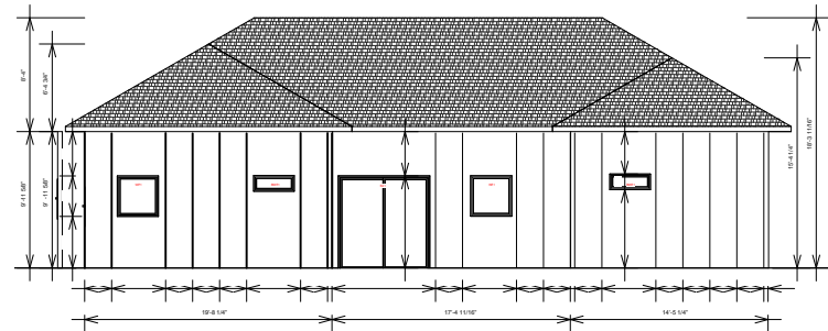
REAR ELEVATION
