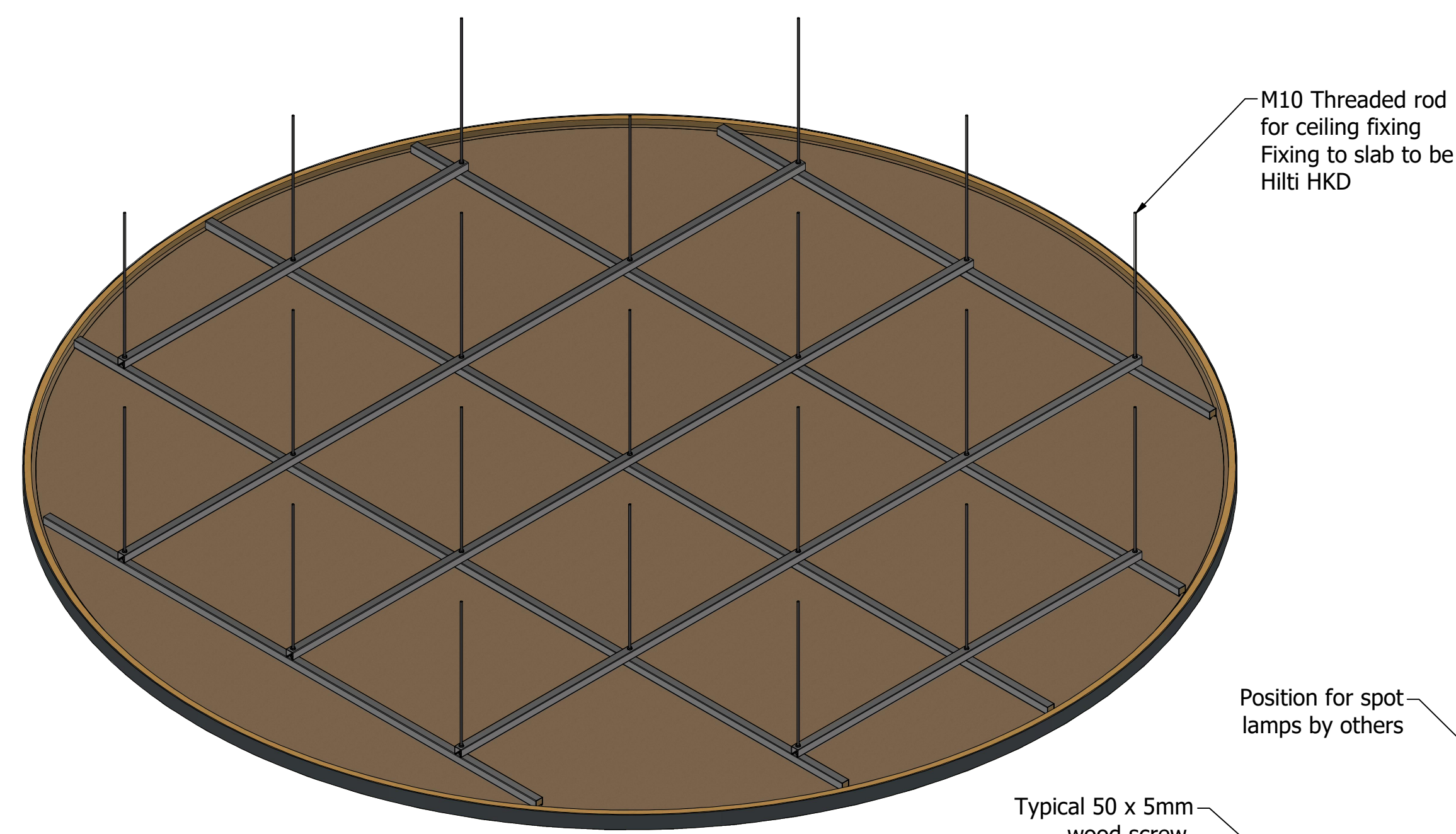
Isometric View Scale 1:20
