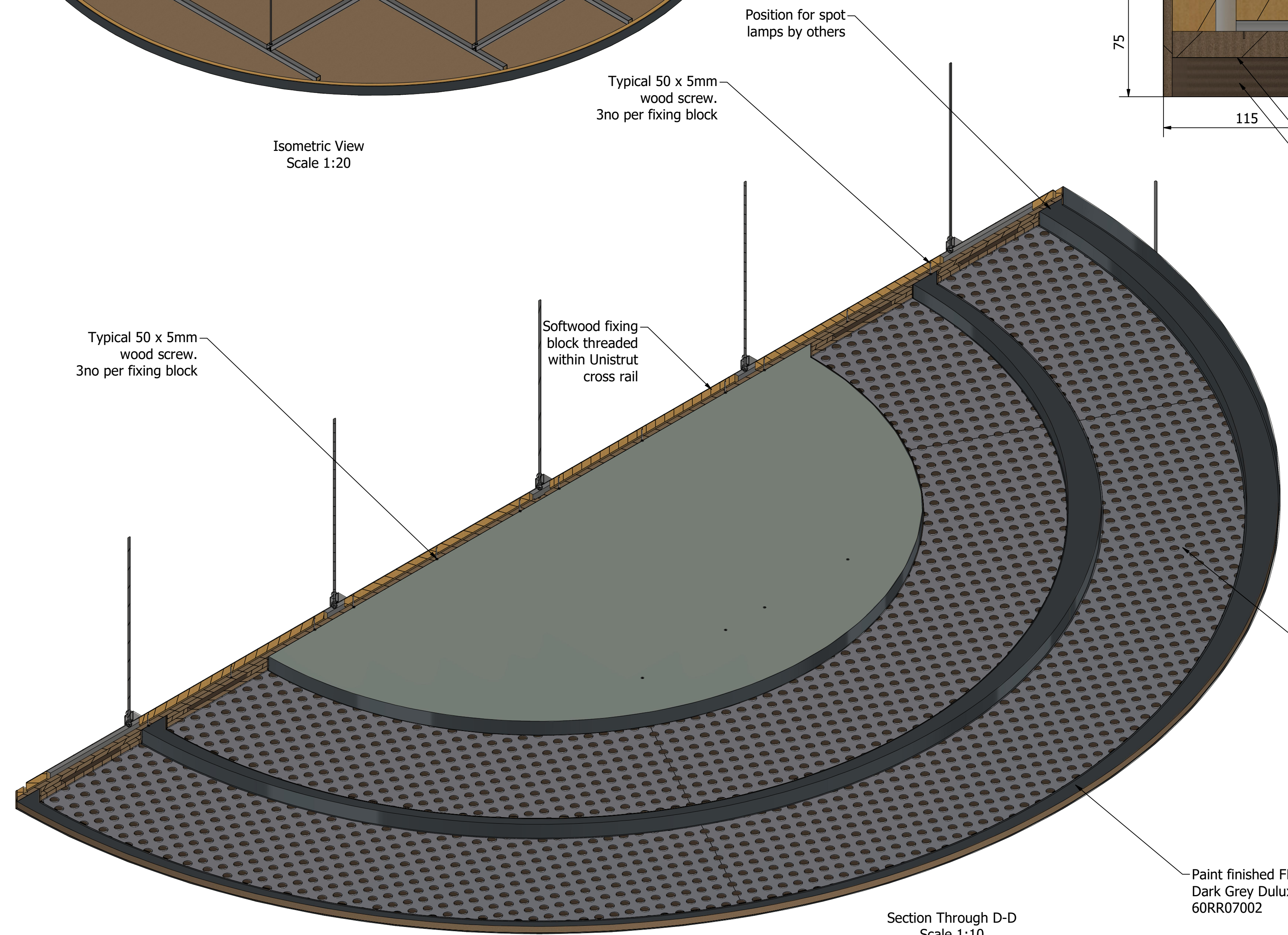
Section Through D-D Scale 1:10
