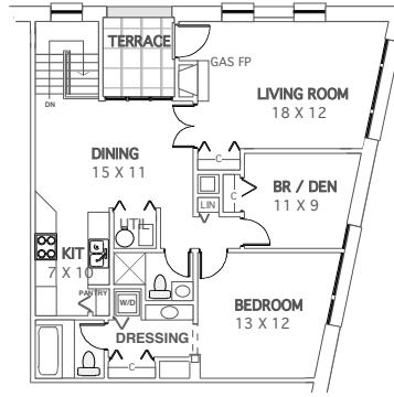
LOWER LEVEL
