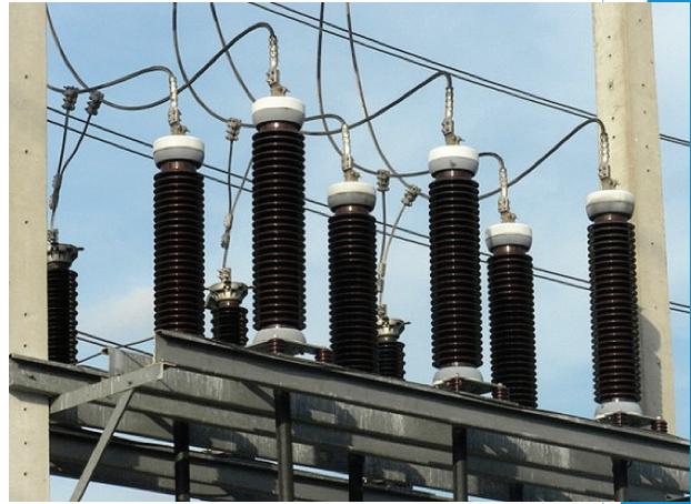
Outdoor terminations with optional brown porcelain.
