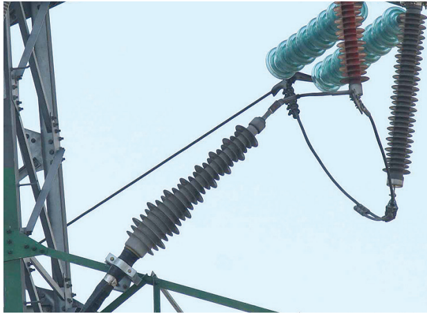
Dry type outdoor termination angle mounted on a tower.
