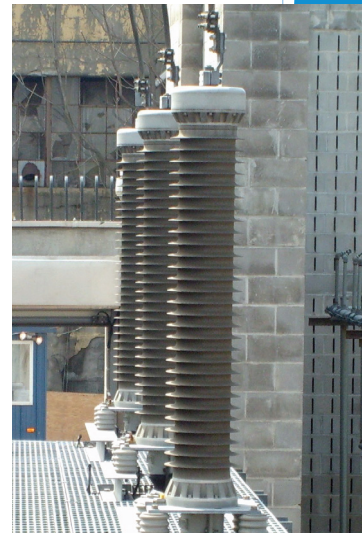
Outdoor termination.
