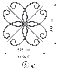
Hand Riveted
