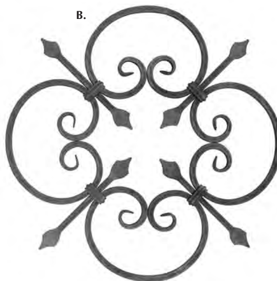
B. 13-1011-3 Forged steel ■ 1/2" (12 mm or .472") Diamond Scored Bar Ø 23-7/8" ±10.69 lbs
