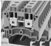
DC10-01P-11-00A(H)
