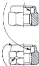
(6) equally spaced stakes plus notch in corner of hex identifies Grade C — inch.
