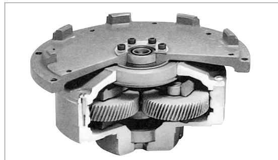
Triple planetary, all-steel gears for smooth power transfer on all models!
