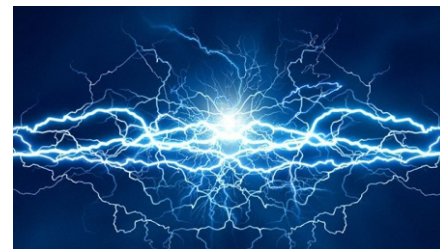
Lightning is one way that nature creates O 3 , ozone.
