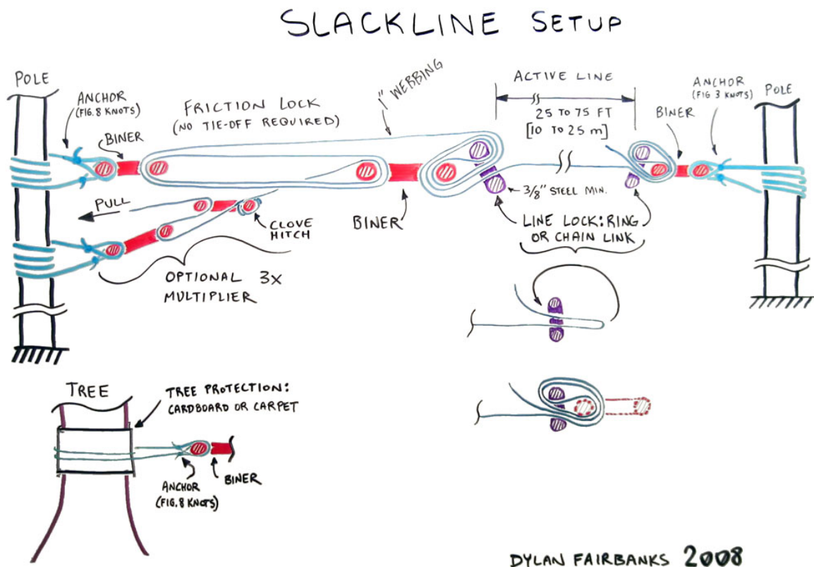
Figure 7: Simple “primitive” slackline set-up
