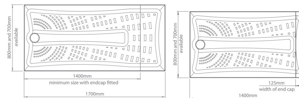
When measuring and cutting the tray please allow for the end cap
