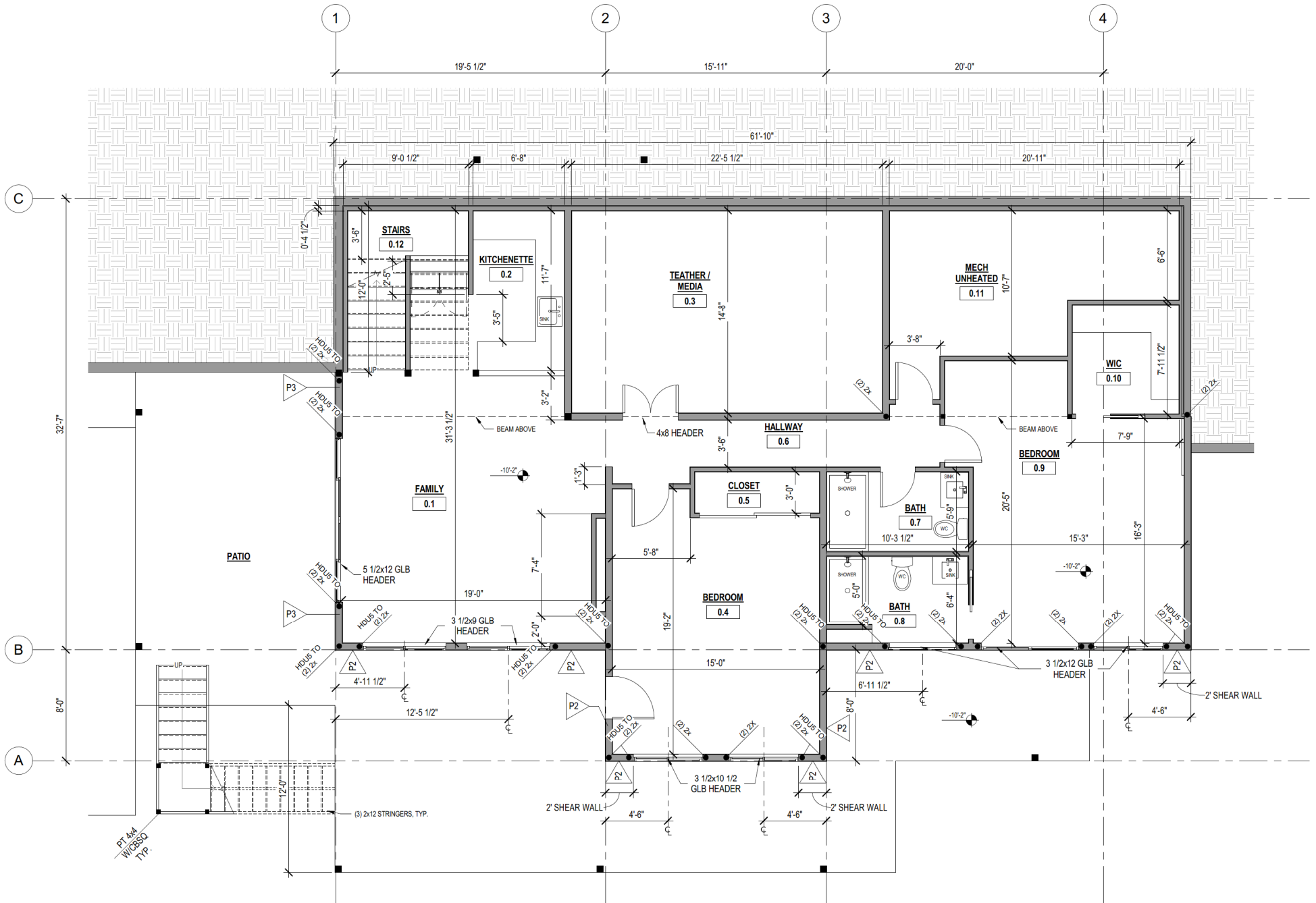
1 Lower Level - Shear Wall Plan 1/4" = 1'-0"
