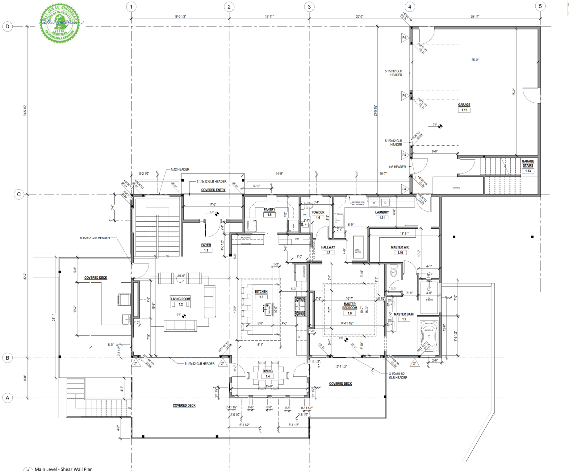
1 Main Level - Shear Wall Plan
