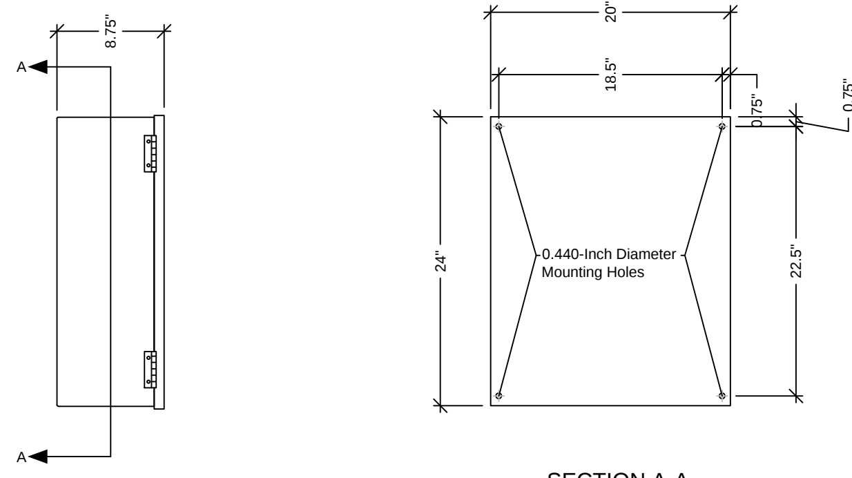
WALL BOX AND MOUNTING HOLE DIMENSIONS No Scale
