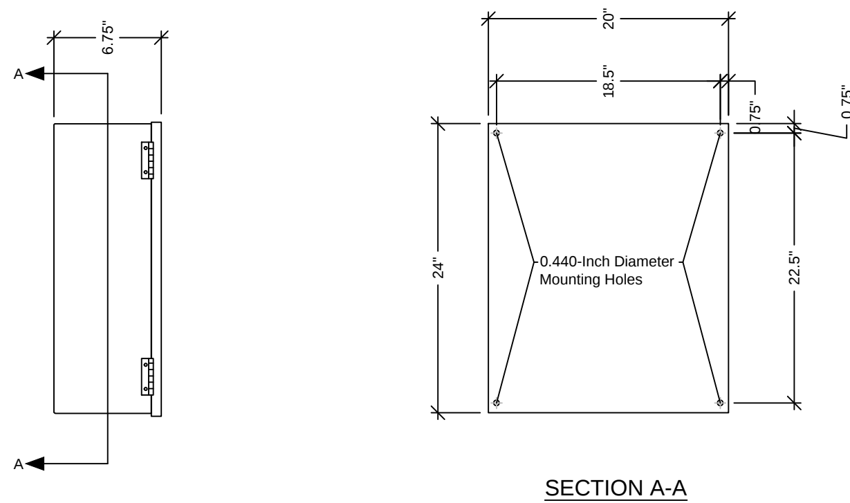
WALL BOX AND MOUNTING HOLE DIMENSIONS No Scale
