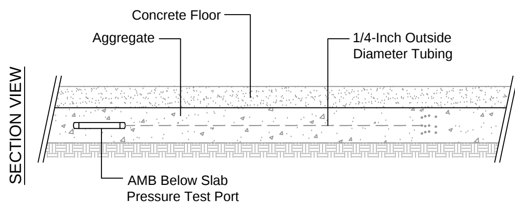
BELOW SLAB PRESSURE TEST PORT WITH FLOOR SAWCUT No Scale
