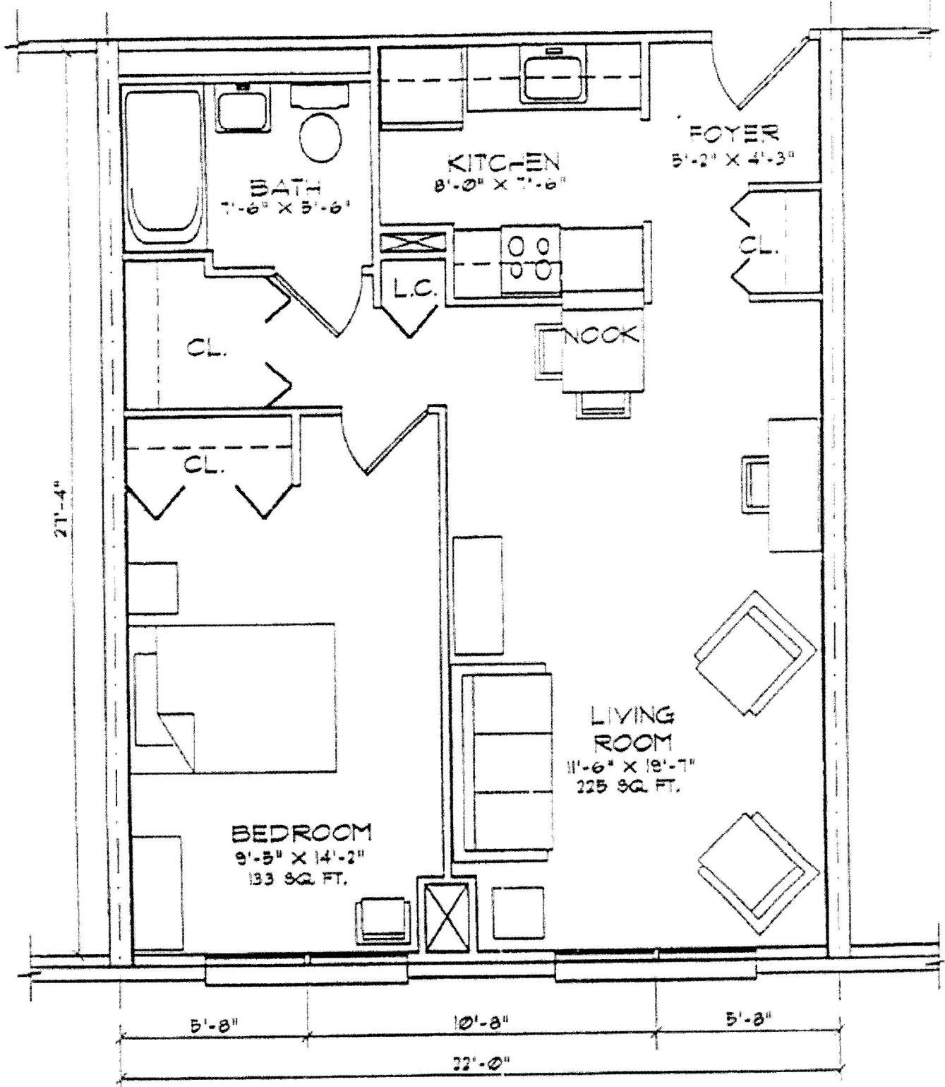
1 TYPICAL UNIT PLAN A-2 V4'-11'-0" 601 SQ. FT. NET
