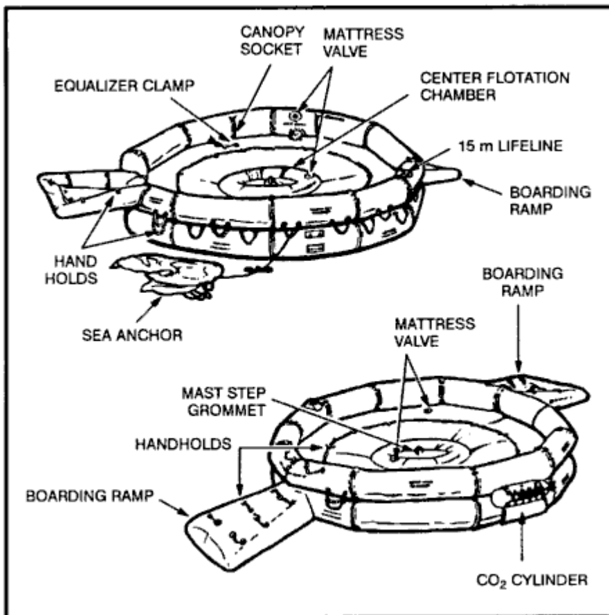
Figure 16-15. Twenty-man raft.
