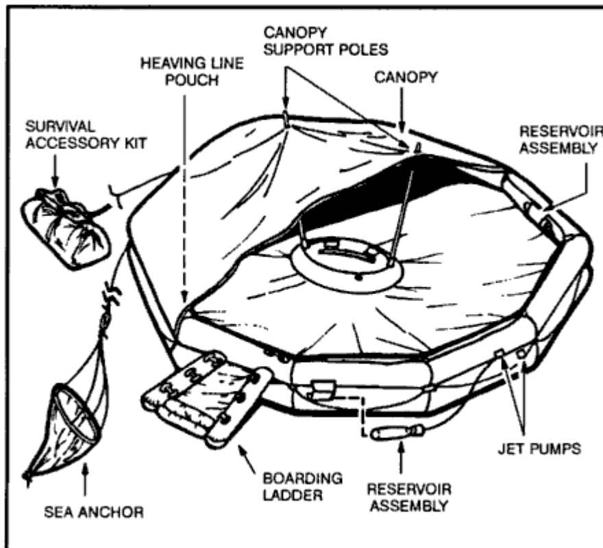
Figure 16-16. Twenty-five-man raft.
