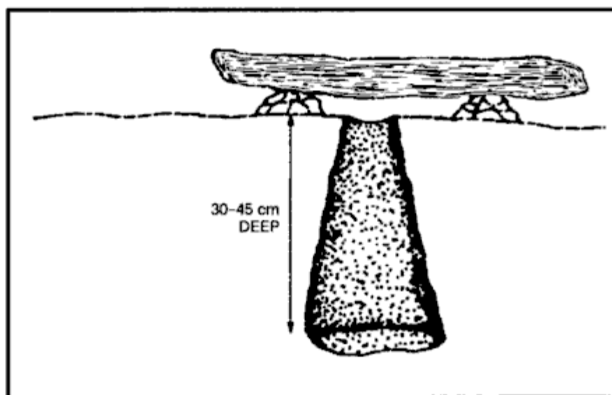
Figure 8-16. Bottle trap.
