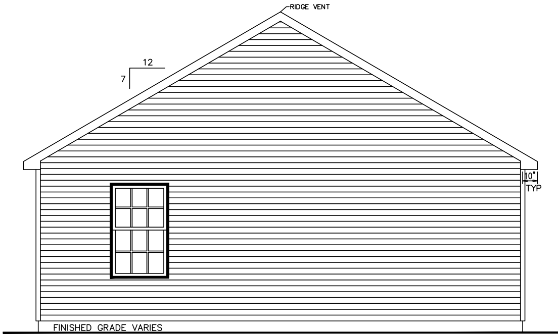
LEFT ELEVATION
