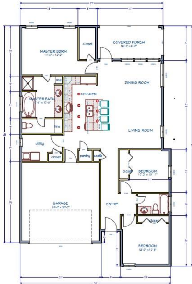
FLOOR PLAN - LIVING AREA 1,610 sqft
