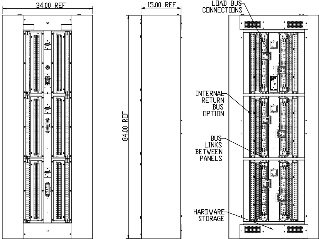
OUTLINE DRAWING OF GROUP 8 (34" WIDE) 7FT CABINET
