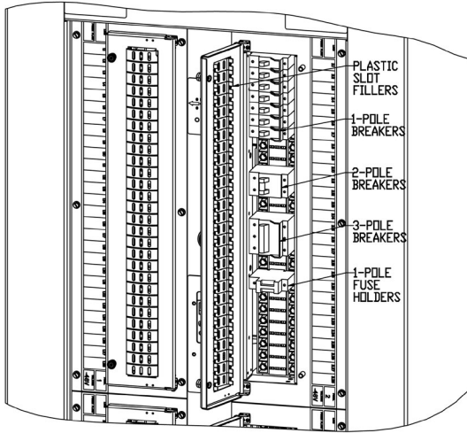
Fuse or Circuit Breaker Installation
