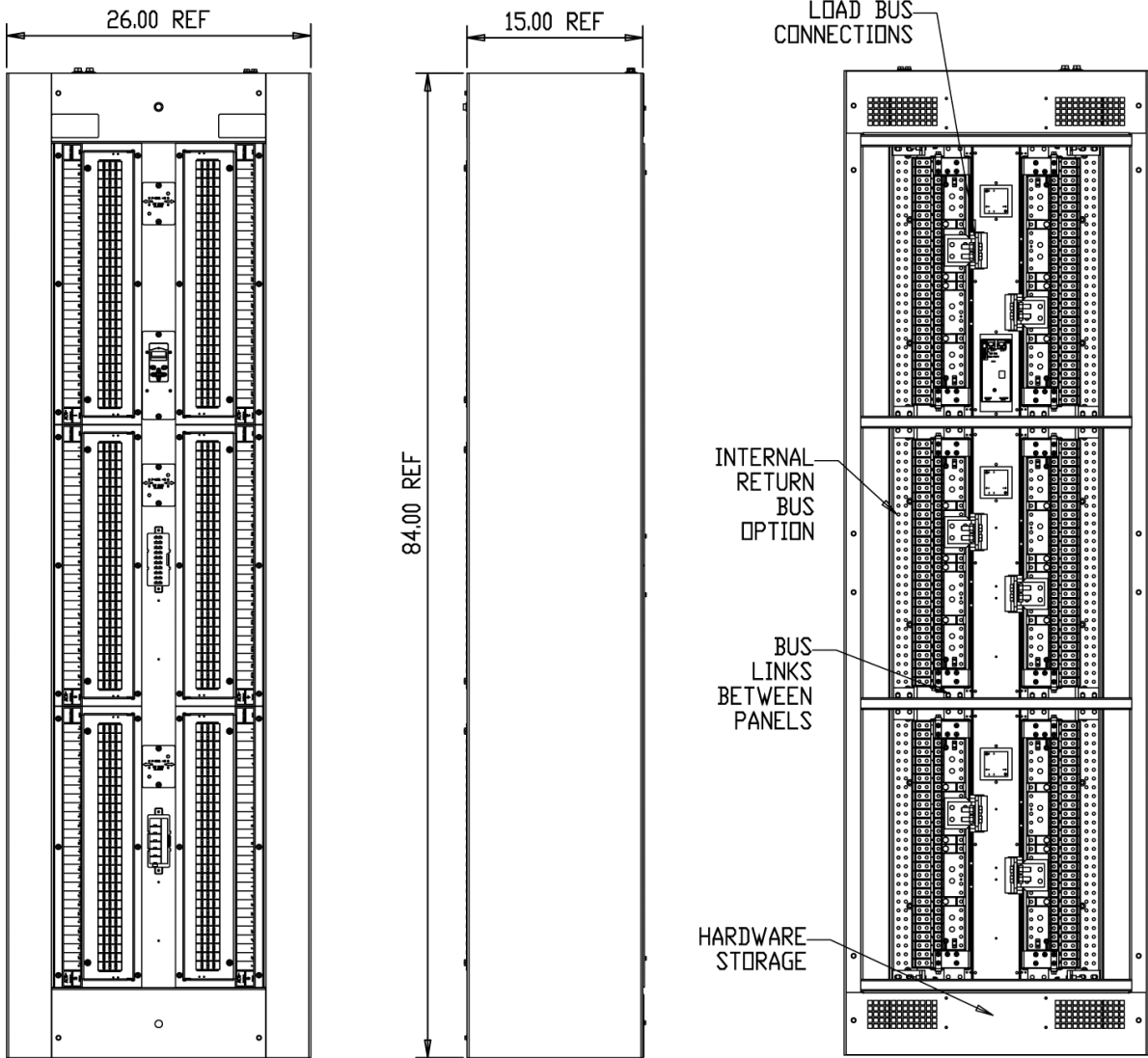
OUTLINE DRAWING OF GROUP 7 (26" WIDE) 7FT CABINET
