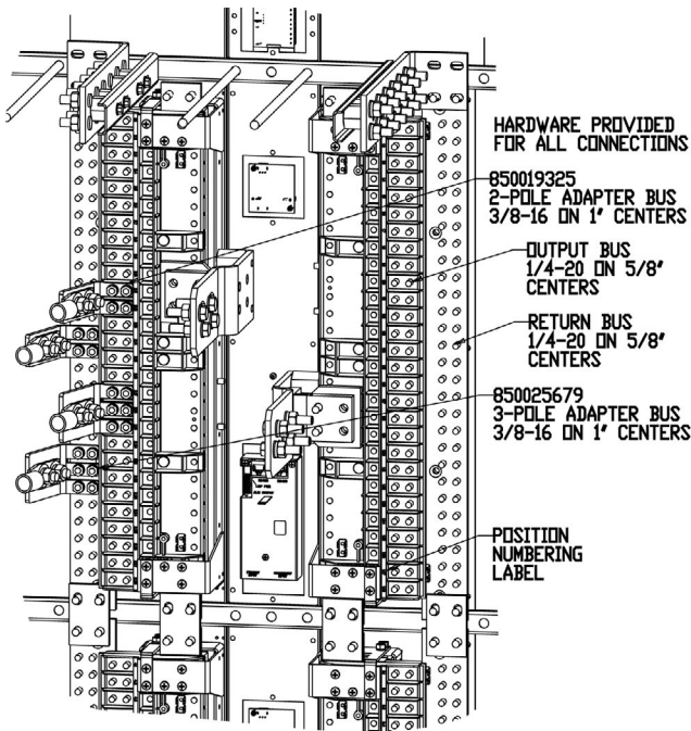
Distribution Panel Connections
