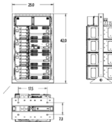
42" high relay rack for mounting 23" wide equipment on a 1/2 height battery stand or battery stack
