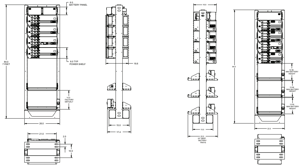
7ft High relay rack for mounting 23" wide equipment
