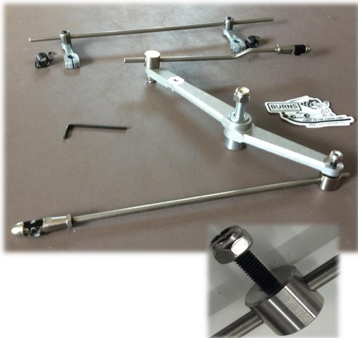
Detail - Swivel - After set screw locates swivel body on rod the lock-nut is adjusted to avoid excess slop.
