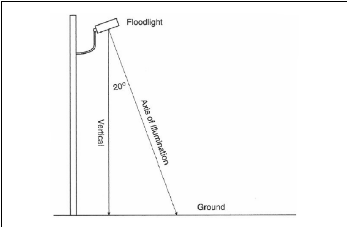
Exhibit 1. The axis of illumination shall be adjusted to an angle not more than 20 degrees from the vertical line between the fixture and the ground.
