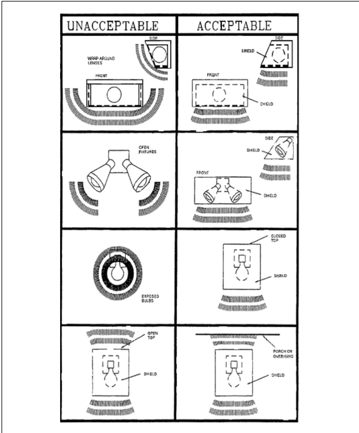
18.1 Fixtures: Diagrams of acceptable and unacceptable fixtures
