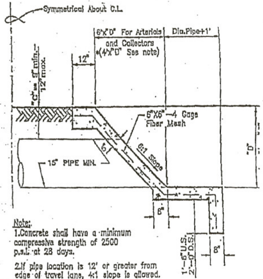
SECTION "B-B"
