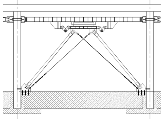
Figure 8. Dampers locations in Y Direction
