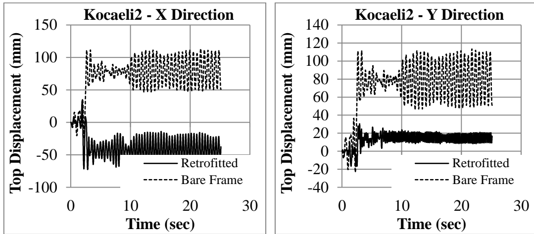
Figure 14. Top Displacement – Time diagram of Kocaeli (1999) - İzmit – 2 earthquake
