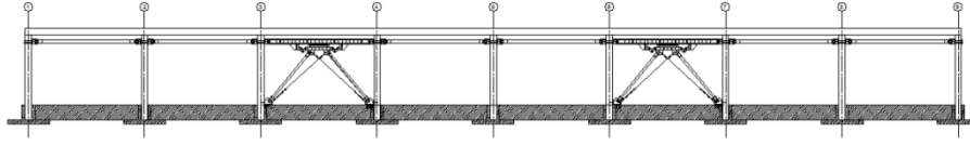
Figure 7. Dampers locations in Y Direction
