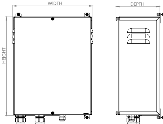
VARCX120 VFD ENCLOSURE
