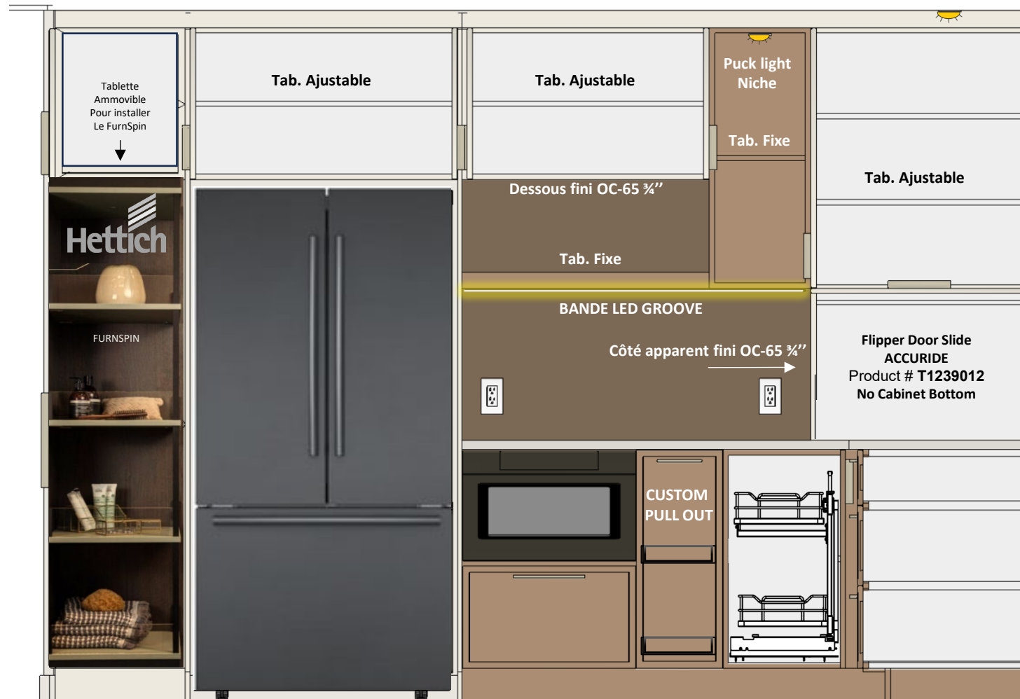
Flipper door - Small appliance storage
