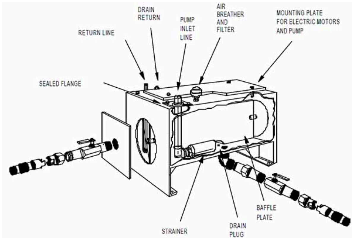
Hydraulic Reservoir Modification
