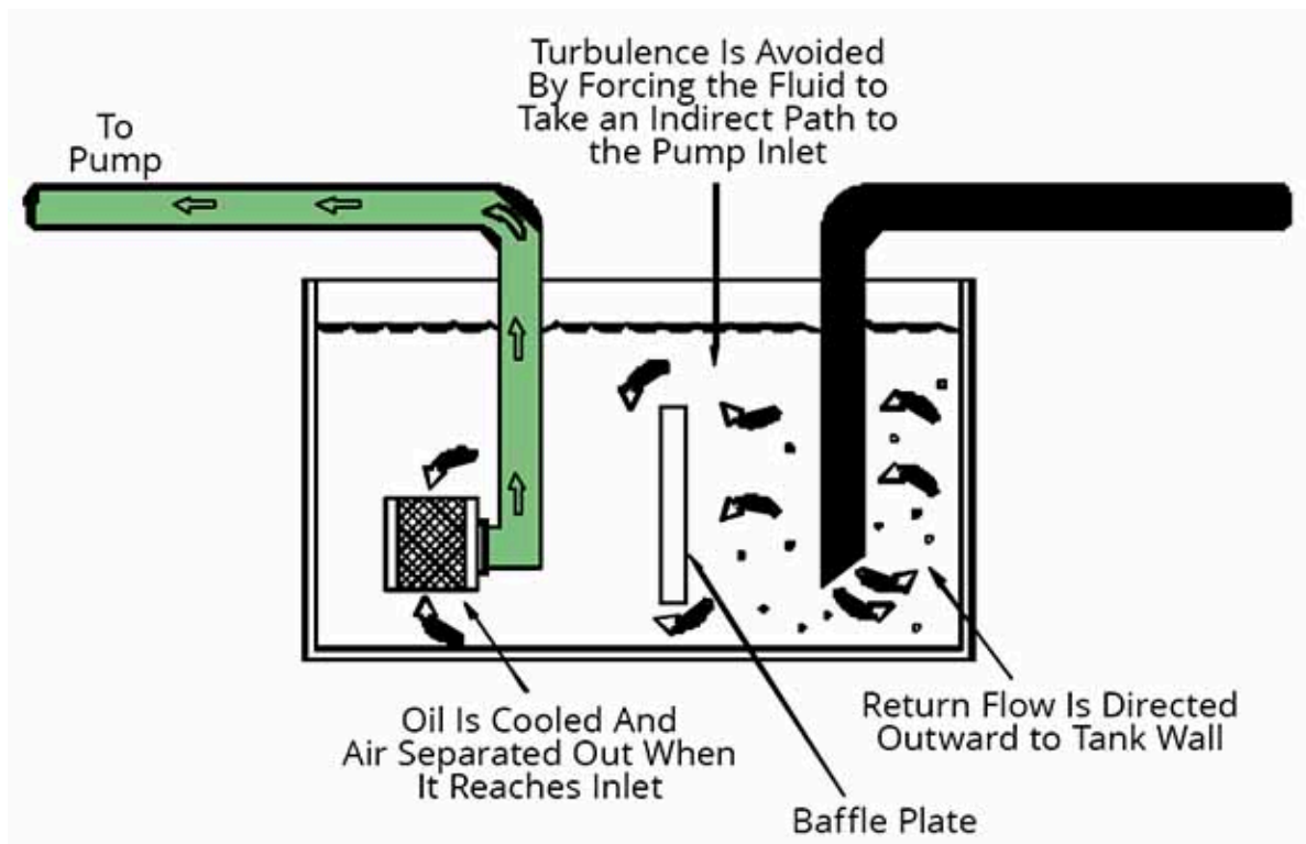
Hydraulic System
