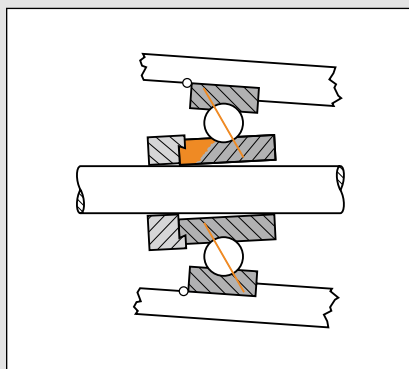
Fig. 62B. Misaligned outer ring.
