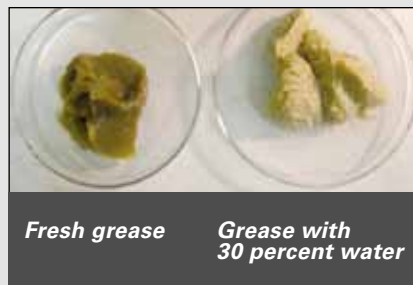
Fig. 73. The effect of water on grease is depicted here.
