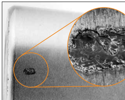
Fig. 59. Electric arc pitting or small burns, magnified 10X here, were created by arcs from improper electric grounding while the bearing was stationary.
