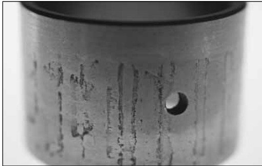
Fig. 11. This cylindrical bearing inner ring has etching and corrosion.
