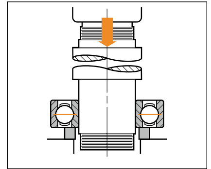
Fig. 54B. Proper mounting procedure on arbor press.
