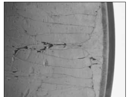
Fig. 57. This cylindrical roller bearing inner ring is crushed by an application failure during service.
