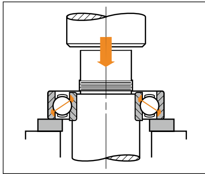
Fig. 54A. Incorrect dismounting of bearing on arbor press.
