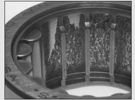
Fig. 37. The housing bore was machined with an improper taper, causing the uneven load distribution and GSC spalling in this cylindrical roller bearing outer ring.
