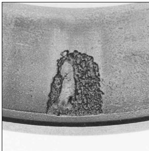
Fig. 48. Localized spalling on this cup race was the result of a stress riser created by a split housing pinch point.
