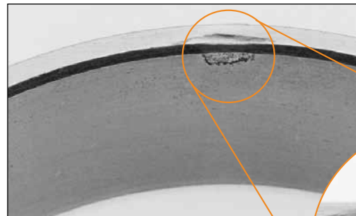
Fig. 40. A hardened driver caused cup face denting on this tapered roller bearing.
