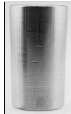
Fig. 38 Rough handling or installation damage resulted in nicks and dents in this tapered bearing roller.
