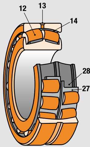
Spherical Roller Bearing
