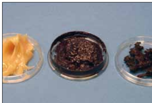
Fig. 71. The above photo shows the same grease at three stages from left to right. 1) new grease, 2) heavily oxidized grease, and 3) worn-out (failed) grease where the thickener and additives have decomposed and the oil has broken down.
