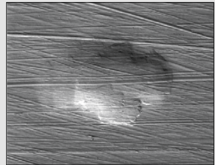
Fig. 8. This photo, taken with a microscope, shows a debris contamination bruise on a bearing race. A corresponding surface map of the dent is shown below in Fig. 10.
