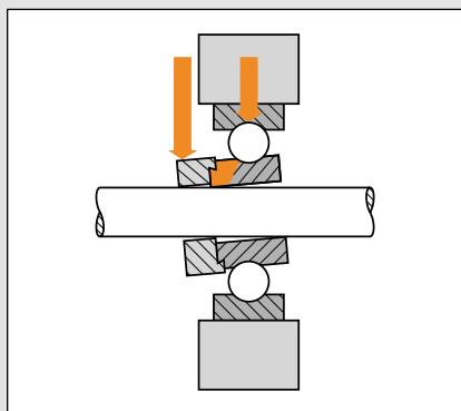
Fig. 62A. Shaft below suggested tolerance levels.
