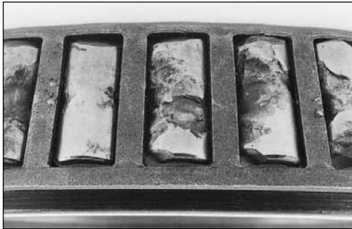
Fig. 29. A heavily overloaded tapered roller bearing resulted in premature, severe fatigue spalling on the rollers. The load was so heavy that large pieces of metal broke off the rollers.
