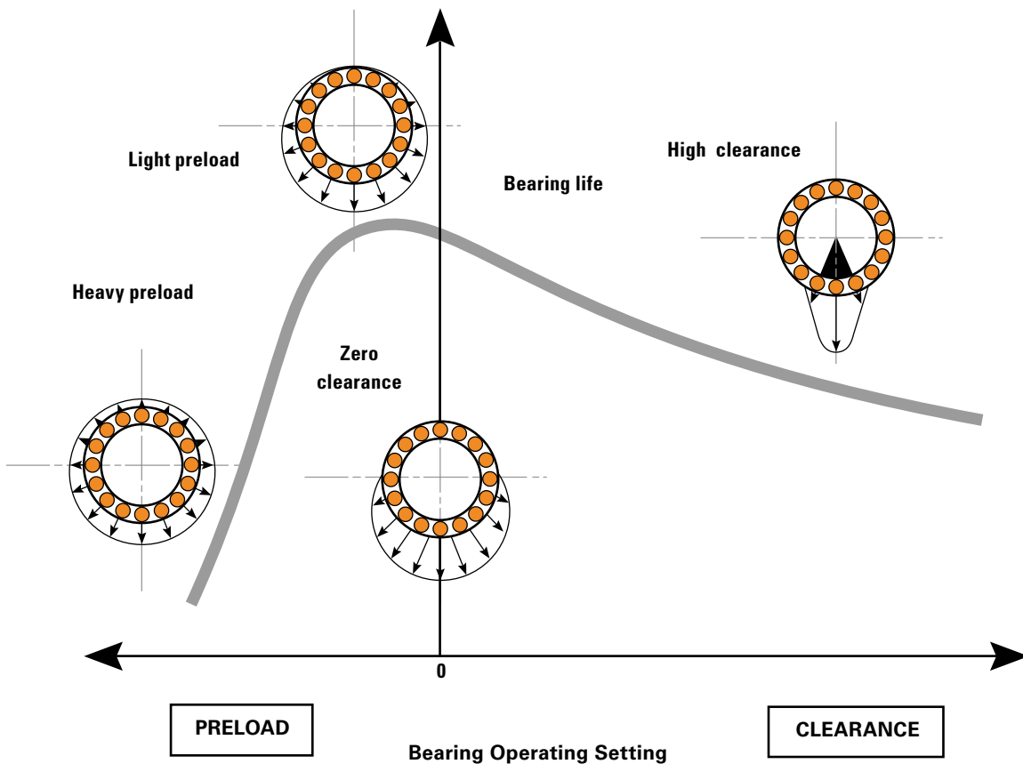
Fig. 63. Bearing life vs. bearing operating setting.
