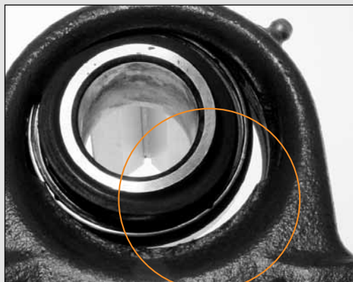
Fig. 2. The roller end wear on this spherical bearing also was caused by fine particle contamination.
