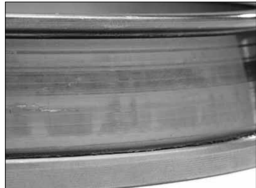
Fig. 16. Level 1 – Discoloration due to elevated operating temperatures.
