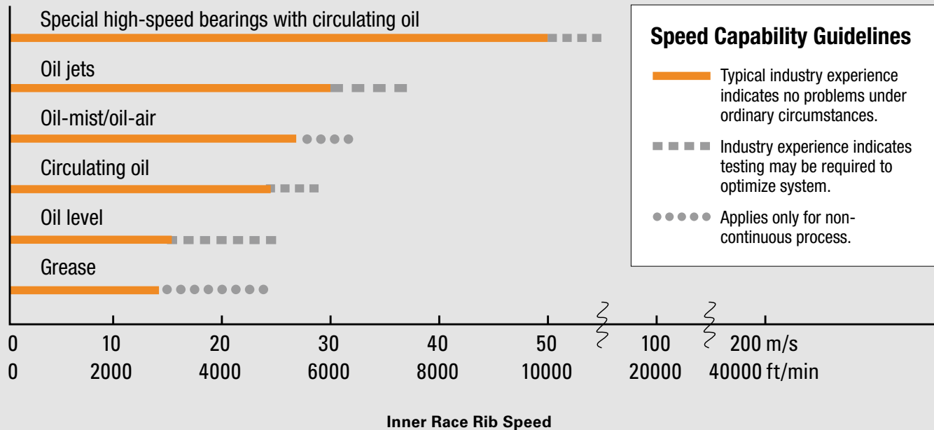
Fig. 79. Here is a summary of guidelines relating to speed and temperature for tapered roller bearings. There are no clear-cut speed limitations for bearings regardless of the bearing design or lubrication systems. The Timken Company recommends that testing be performed for all new high-speed applications, regardless of bearing design.
