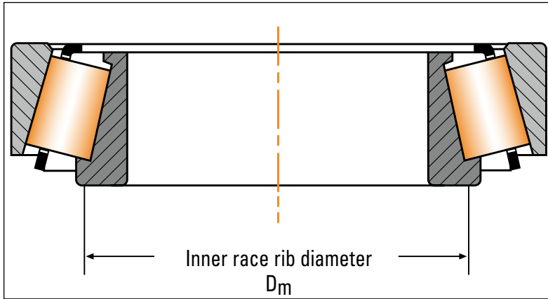
Fig. 78. The inner race rib diameter can be scaled from a drawing or can be approximated as the average of the bearing inner and outer diameter.
