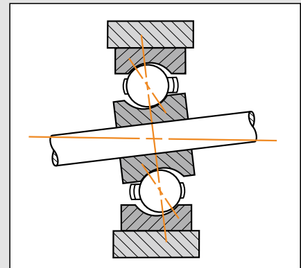
Fig. 34A. Shaft misalignment
