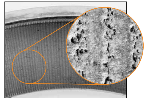
Fig. 61. Magnified 10X, this fluting, defined as a series of small axial burns, was caused by an electric current passing through the bearing while it was rotating.
