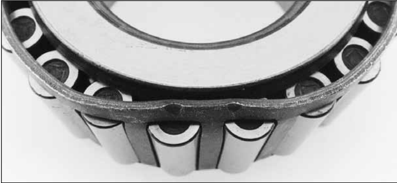
Fig. 42. This cage deformation was caused by an improperly installed or dropped bearing.
