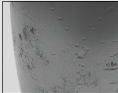
Fig. 7. Hard particles caused contamination bruising on this spherical roller bearing.
