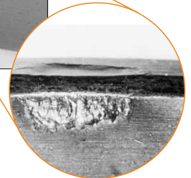
Fig. 40. A hardened driver caused cup face denting on this tapered roller bearing.
