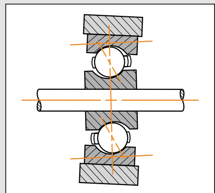
Fig. 34B. Housing misalignment
