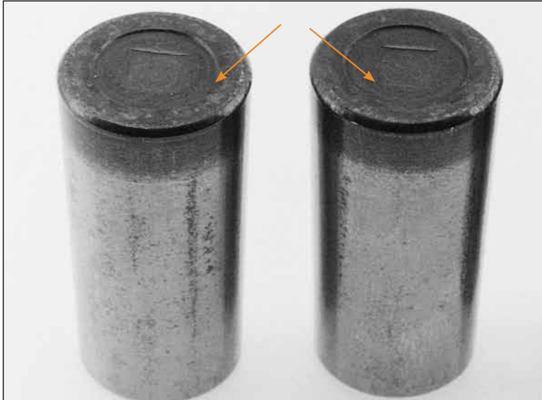
Fig. 19. Level 3 – Heat damage on these tapered rollers was caused by metal-to-metal contact.
