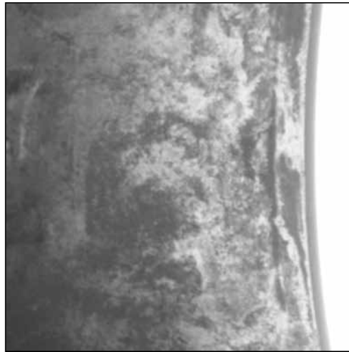
Fig. 46. Classic fretting corrosion from poor fitting practice is depicted here. Relative movement under load between the bearing and its seat caused this worn and corroded condition.
