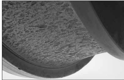
Fig. 30. Severe peeling and spalling is shown on this spherical bearing race, also resulting from high loads.
