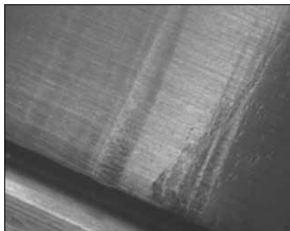
Fig. 55. This inner ring of a spherical roller bearing shows roller impact damage from shock loading.
