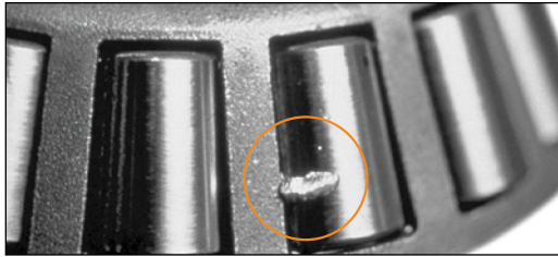
Fig. 5. Large particle contamination imbedded into the soft cage material can result in grooving.
