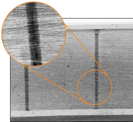
Fig. 53. A heavy impact load on this tapered bearing cup race caused brinell and impact damage. These same indentations are evident on the cone race. This is true metal deformation and not wear as with false brinelling. The close-up view of one of the grooves shows the grinding marks still in the groove.
