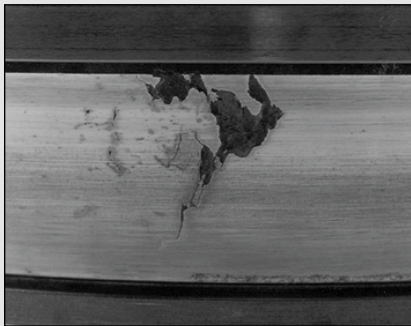
Fig. 6. A tapered roller bearing inner race (cone) with spalling from debris contamination bruises.
