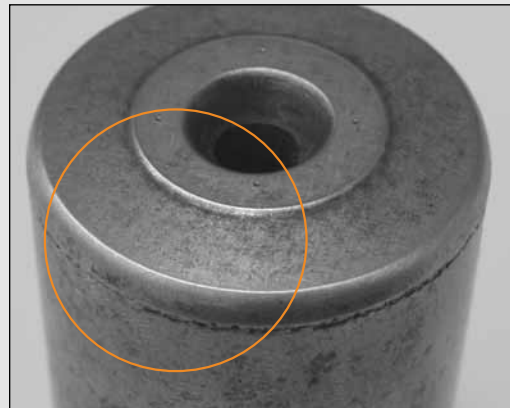
Fig. 2. The roller end wear on this spherical bearing also was caused by fine particle contamination.
