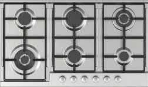
9LEE4G2T 90 CM STAINLESS STEEL BUILT IN HOB BURNERS: 4 GAS AND 2 WOK BURNER GAS CONTROL UNDERKNOB AUTO IGNITION
