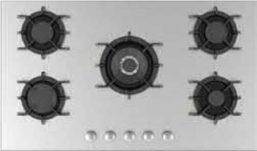
9ST4GT 90 CM STAINLESS STEEL BUILT IN HOB BURNERS: 4 GAS AND 1 WOK BURNER GAS CONTROL UNDERKNOB AUTO IGNITION
