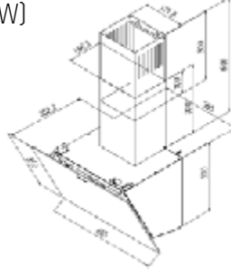
W50MIDCTBL3,2 Wall Mounted Hood Black Paint Body & Black Glass Model Lightining: 2xSpot LED (2*2W)
