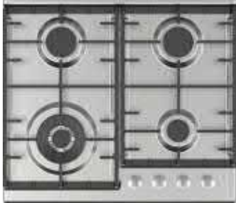
6LD3GT 60 CM STAINLESS STEEL BUILT IN HOB BURNERS: 3 GAS AND 1 WOK BURNER GAS CONTROL UNDERKNOB AUTO IGNITION
