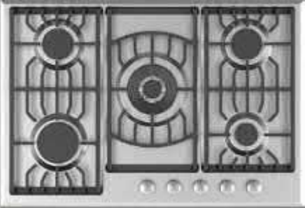
7LSP4GT 70 CM STAINLESS STEEL BUILT IN HOB BURNERS: 4 GAS AND 1 WOK BURNER GAS CONTROL UNDERKNOB AUTO IGNITION
