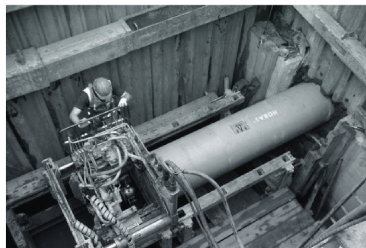
Jacking Pipe / Slip-Lining
