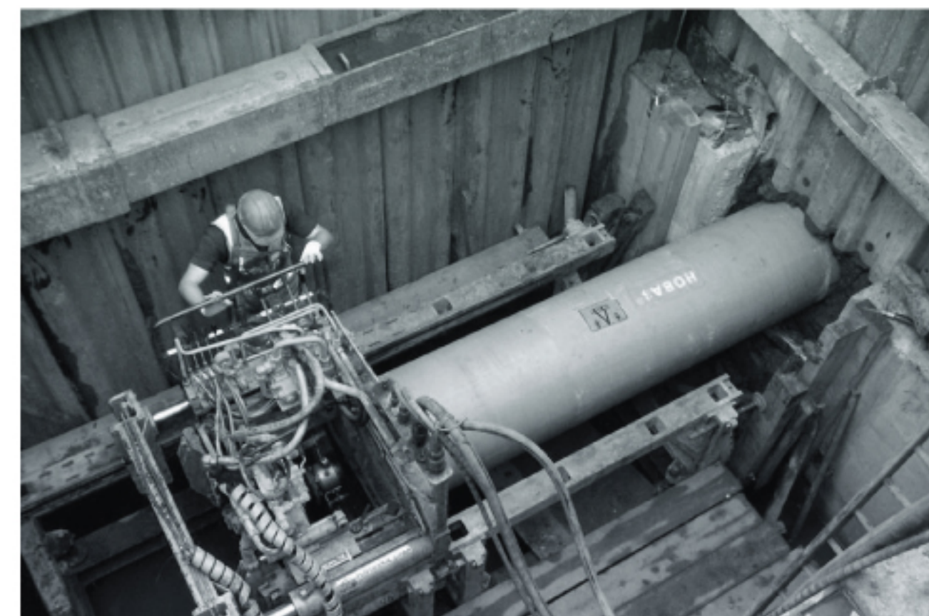
Jacking Pipe / Slip-Lining
