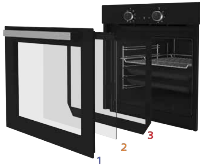
Triple Glass Oven Door
